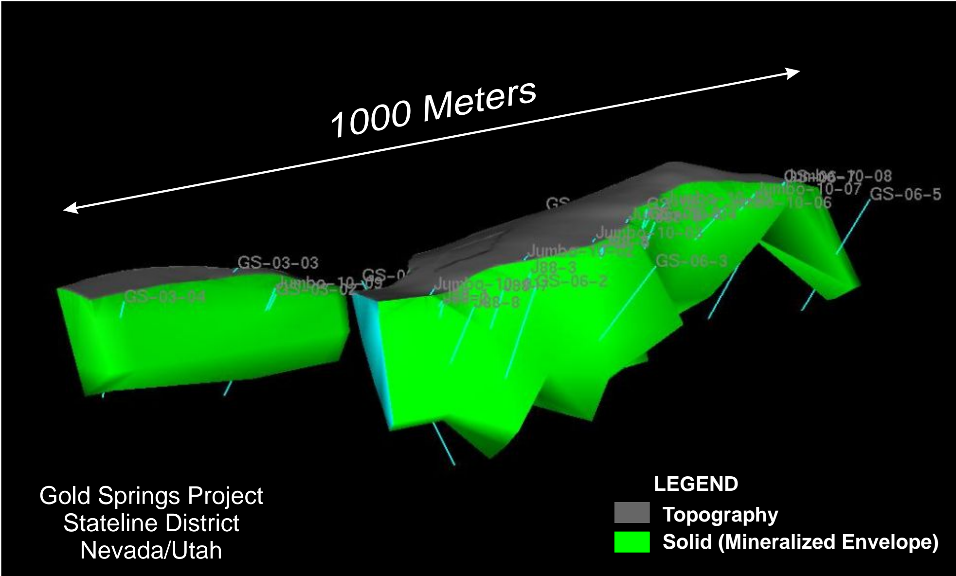
Jumbo Area 3D View Showing Mineralized Envelope View Looking Northwest
