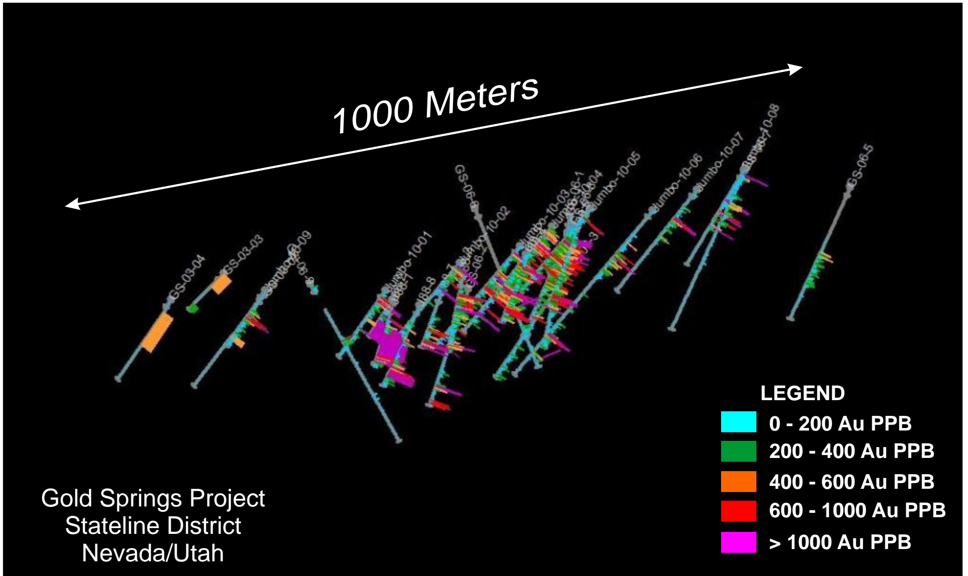
Jumbo Area 3D View Showing Drill Holes Assays in ppb View Looking Northwest
